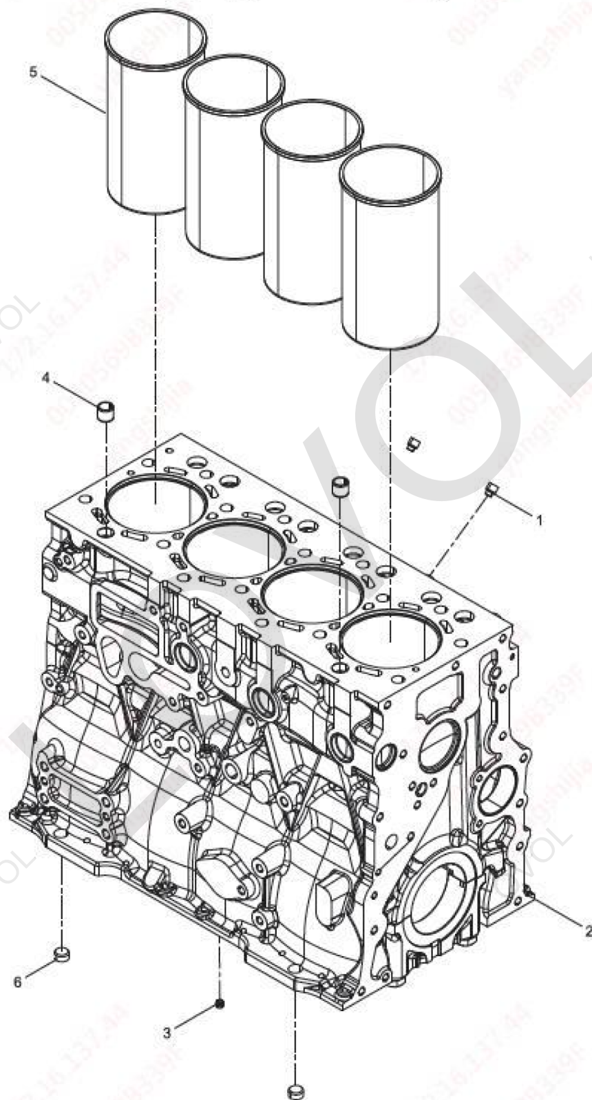
机体总成(Crankcase Assembly)
