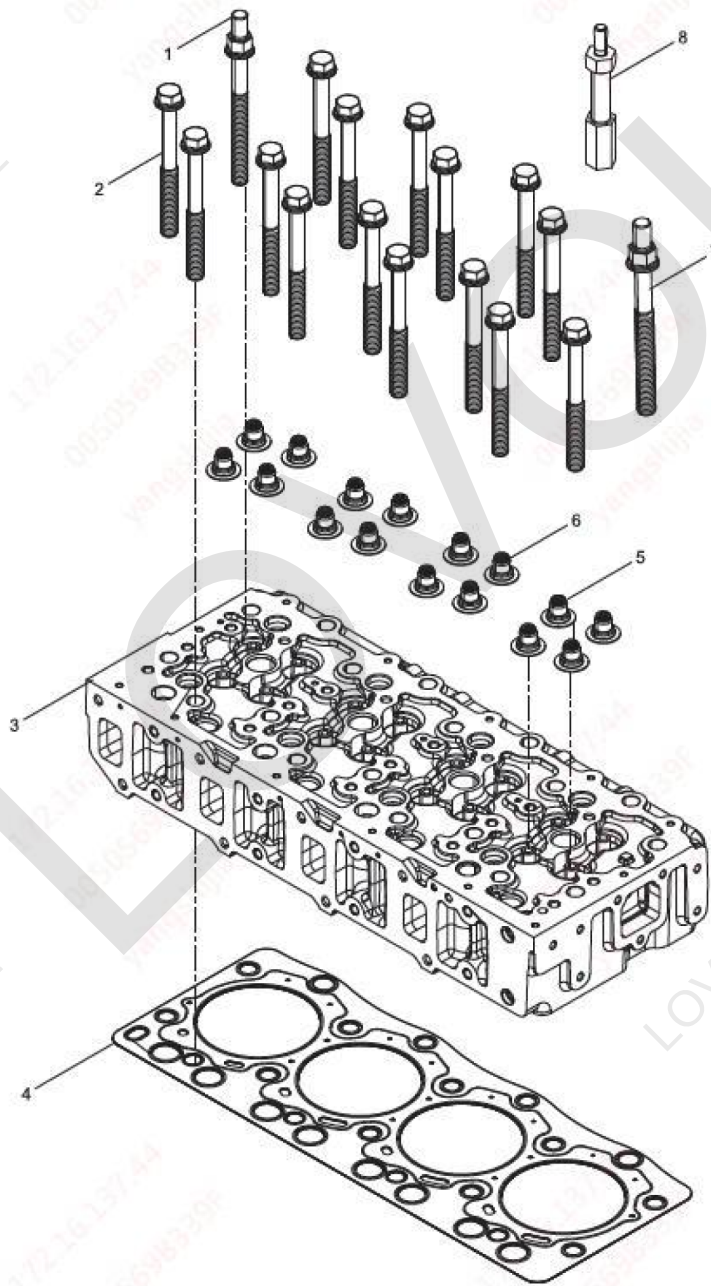
气缸盖结合组(Cylinder Head Group)
