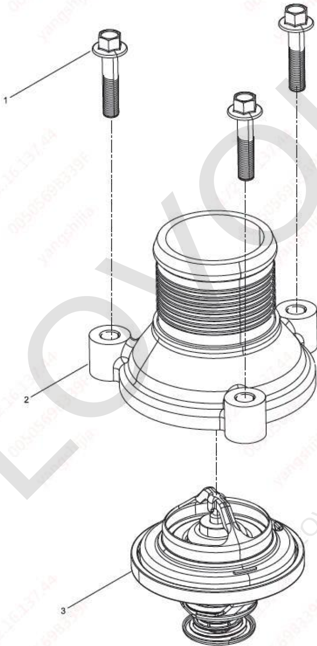
节温器结合组(Thermostat Group)
